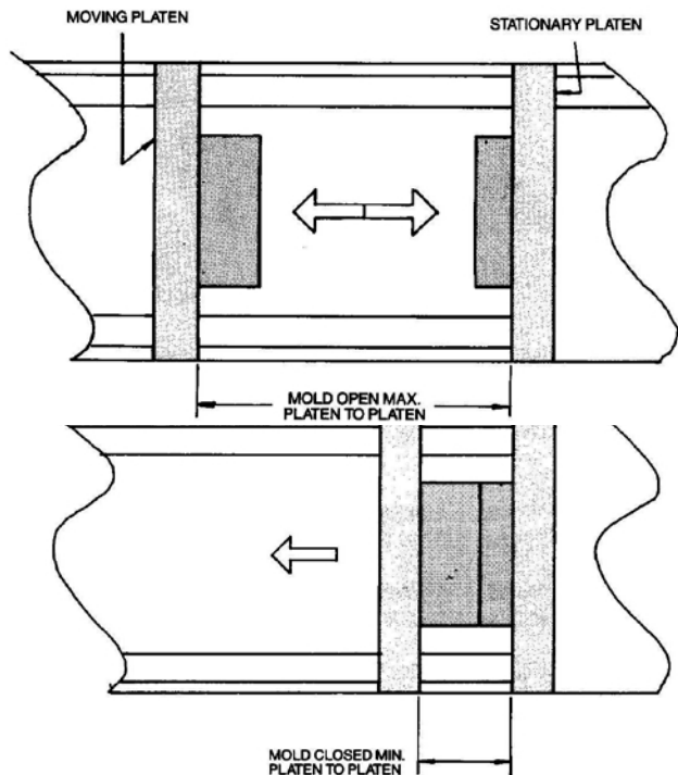
Mold Open position
