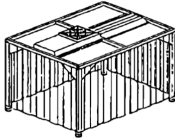
"B" - 8 INCH STRIP CURTAINS WITH 2 INCH OVERLAP
